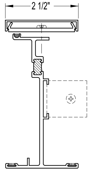
#L1000T-M1, M2 / M3 FOR 4 1/2" WINDOW SYSTEMS
