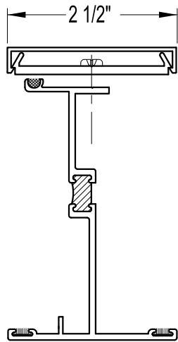
#L500T-M1, M2 / M3 FOR 3 3/4" WINDOW SYSTEMS
