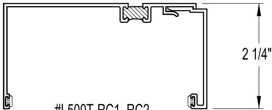
#L500T-RC1, RC2 FOR 3 3/4" WINDOW SYSTEMS
