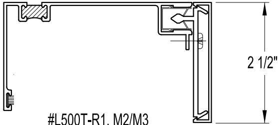
#L500T-R1, M2/M3 FOR 3 3/4" WINDOW SYSTEMS
