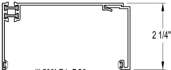
#L500I-R1, RC2 FOR 3 3/4" WINDOW SYSTEMS
