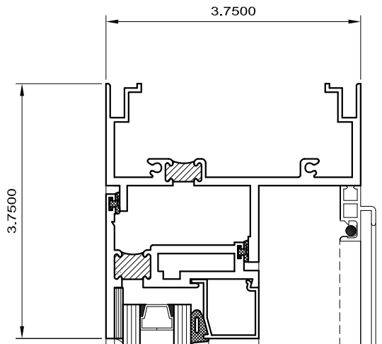
1 HEAD
