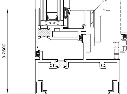
2 SILL
