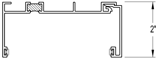
STANDARD HEAD / JAMB RECEPTOR FOR 3 3/4" WINDOW SYSTEMS
