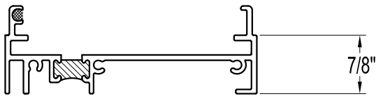
STANDARD STARTER SILL FOR 3 3/4" WINDOW SYSTEMS
