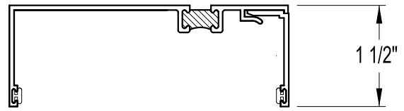
HEAD / JAMB RECEPTOR FOR 3 3/4" WINDOW SYSTEMS
